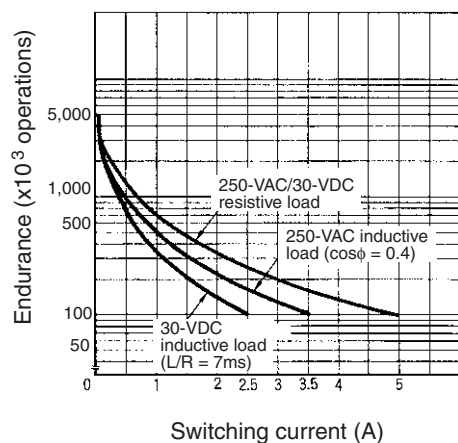
Fully sealed Relays G2R-14, G2R-1A4
